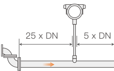
Two 90° elbows in one plane
