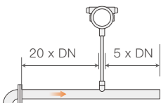
One 90° elbow
