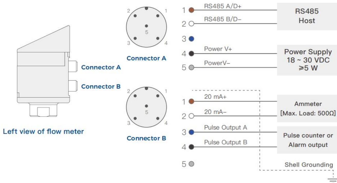
Figure 3-7 Flow Meter Connection
