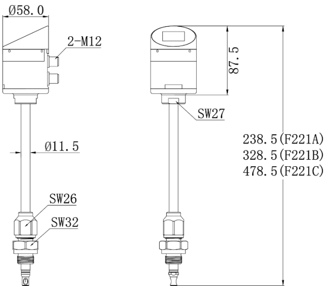
Figure 3-3 F211x Dimension Diagram
