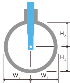
Figure 3-4 Diagram of Measuring Point Selection
