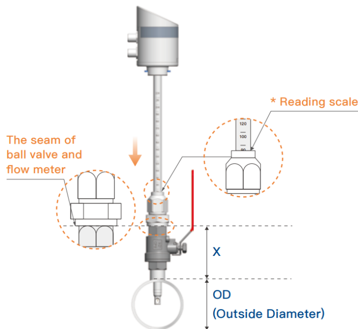
Figure 3-6 Diagram of Insertion Depth Calculation
