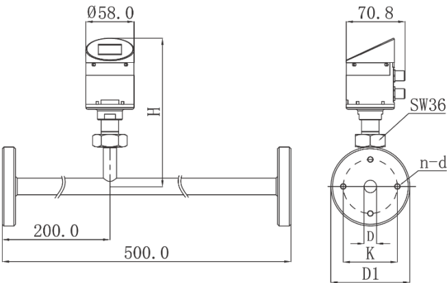
Figure 3-2 F222x Flange-type Dimension Diagram
