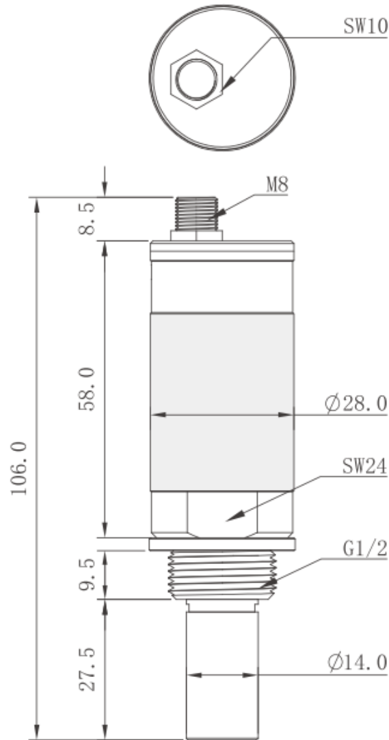
Figure 3-1 F113x Series Dimension Diagram
