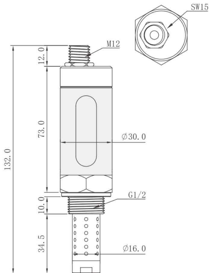
Figure 3-1 F108x Series Dimension Diagram
