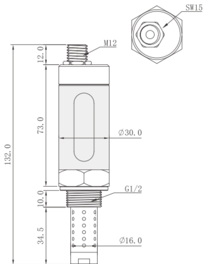
Figure 3-1 F103x Series Dimension Diagram
