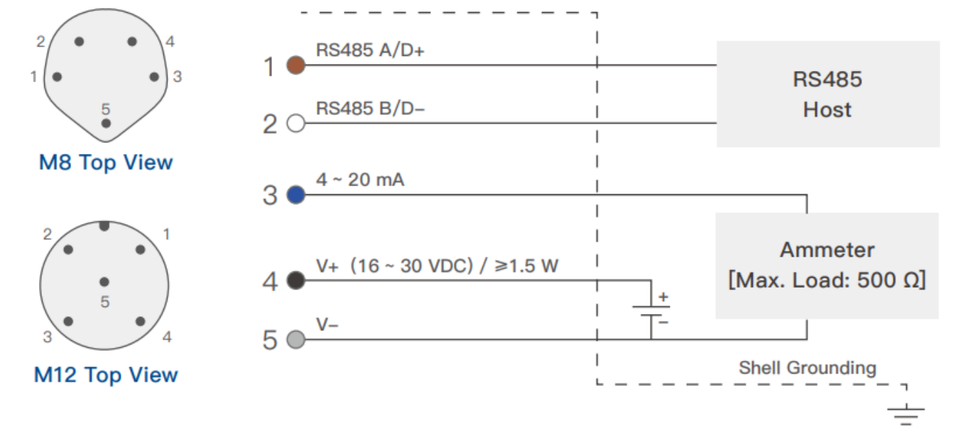
Figure 3-4 Electrical Connection Diagram
