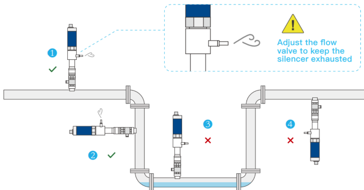
Figure 3-2 Installation with Measuring Chambers
